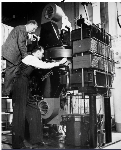
Vacuum chamber of GE synchrotron
