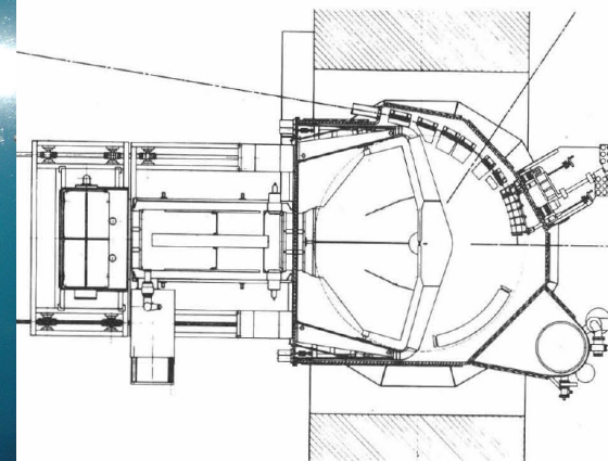
Fig.8. Top view
