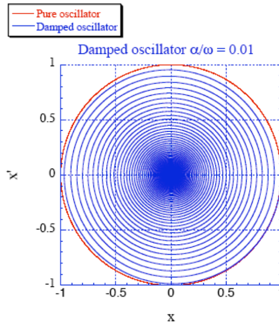
Fig. 17-1 Poincaré plot of trajectories of normal and damped oscillator in dimensionless coordinates x/a ; x'/\omega a .
