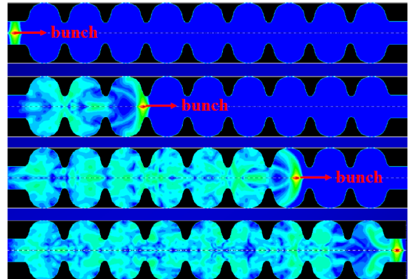
Fig. 17-3 A couple picture of wakefield generated by charged particles
