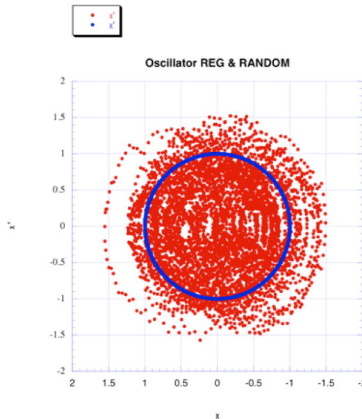
Fig. 17-2 Poincaré plot of trajectories of normal and damped oscillator with random kicks (in dimensionless coordinates x/a ; x'/\omega a ).
