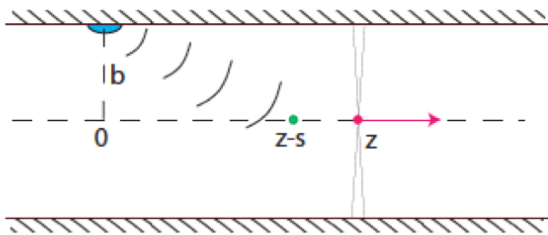
Fig. 17-3 A couple picture of wakefield generated by charged particles
