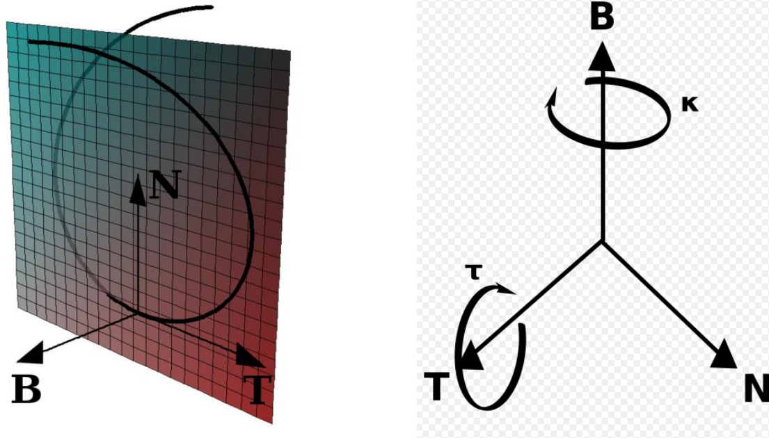
Fig. 2. Illustration of Frenet-Serret formulas and system from http://en.wikipedia.org/wiki/Frenet-Serret
