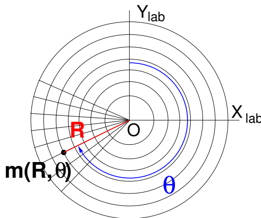
Fig. 1.7 A sketch of a cylindrical field map mesh, i.e., a set of m(R, \theta) nodes in a frame (O, X, Y) , covering 180^\circ (solid lines). The median plane field map so defined, namely the set of vertical field component values B_z(R, \theta) at the nodes of the mesh, represents a half of the cyclotron dipole; using it twice (additional 180^\circ dashed line mesh) allows covering the all 360^\circ dipole. The mesh nodes are distant \Delta R radially, \Delta\theta in angle. Note: fabricating a 2D median plane field map is an easy way to define a magnetic field distribution for ray-tracing, often useful when an accurate analytical modeling is not available at hand.
