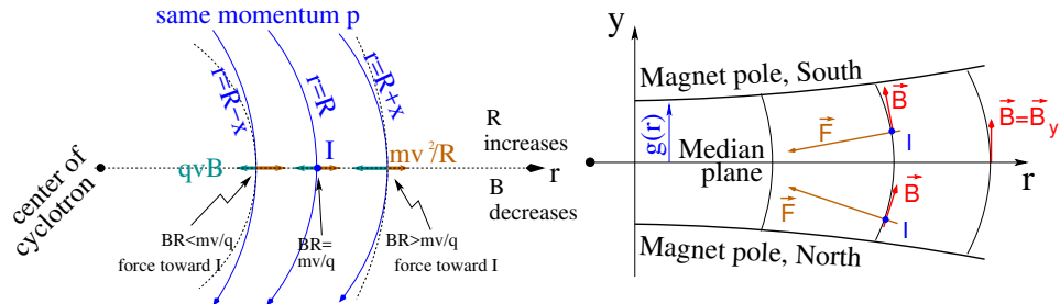
Fig. 1.10 Motion stability in a weak focusing axially symmetric structure. Left, radial: the resultant of the bending and outward forces pulls particles with momentum p = mv toward the equilibrium orbit at R = p/qB , resulting in a stable oscillation around the latter. Right, axial: positive ions off the median plane (at I, coming out of the page) experience a force pulling toward the median plane. Note the hyperbolic shape of the gap g(r) = g_0(r_0/r)^k , creating the field B(r) = B_0(r/r_0)^k , Eq. 1.9.
