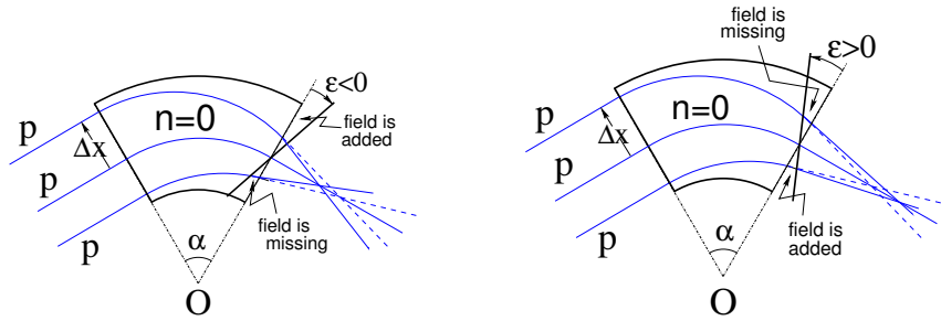
Fig. 1.15 Left: a focusing wedge ( \epsilon < 0 by convention), opening the sector augments the horizontal focusing. Right: a defocusing wedge ( \epsilon > 0 by convention), closing the sector diminishes the horizontal focusing. Focal distance in the bend plane respectively decreases, increases. The reverse holds in the vertical plane, opening/closing the sector decreases/increases the vertical focusing.
