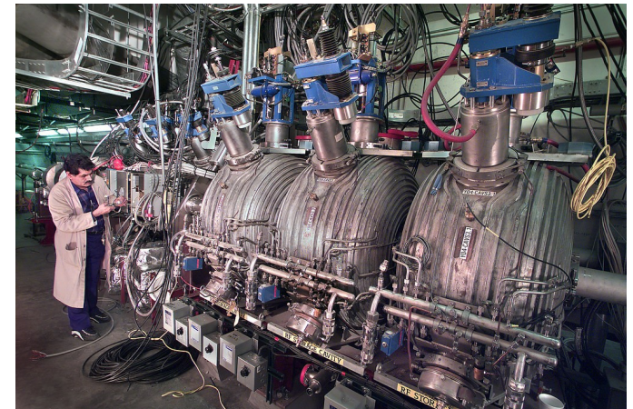
RF cavities of AGS - 25 GeV ring
