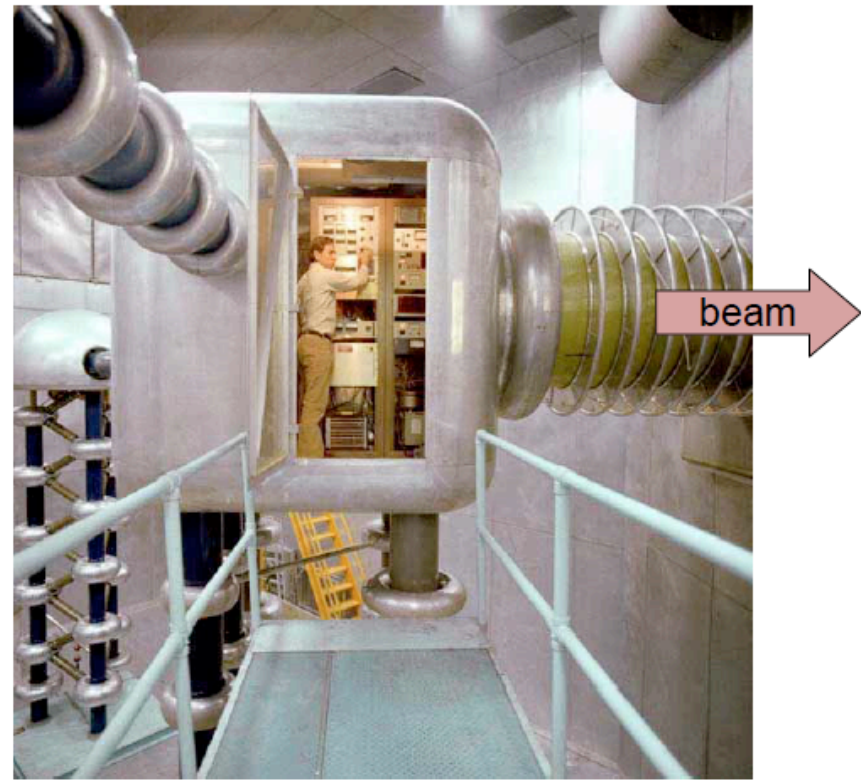
Crockroft-Walton at FNAL accelerates H - to 750keV
