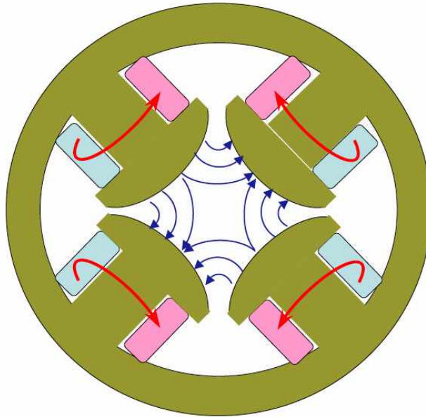
Fig. 2.17. Typical quadrupole magnet.
