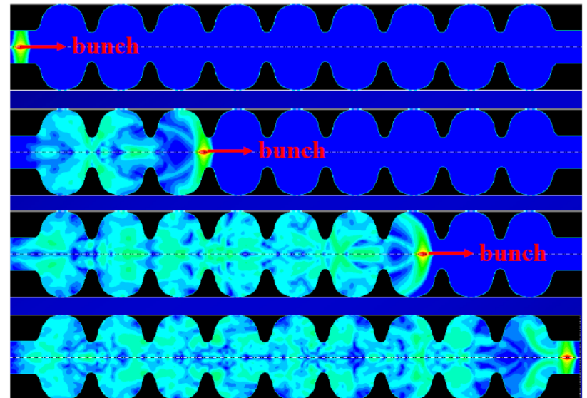
Fig. 3, A couple picture of wakefield generated by charged particles
