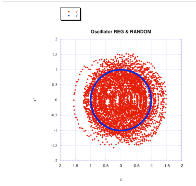
Fig. 2 Poincaré plot of trajectories of normal and damped oscillator with random kicks (in dimensionless coordinates x/a ; x'/\omega a ).
