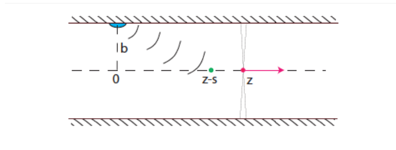
Fig. 3, A couple picture of wakefield generated by charged particles
