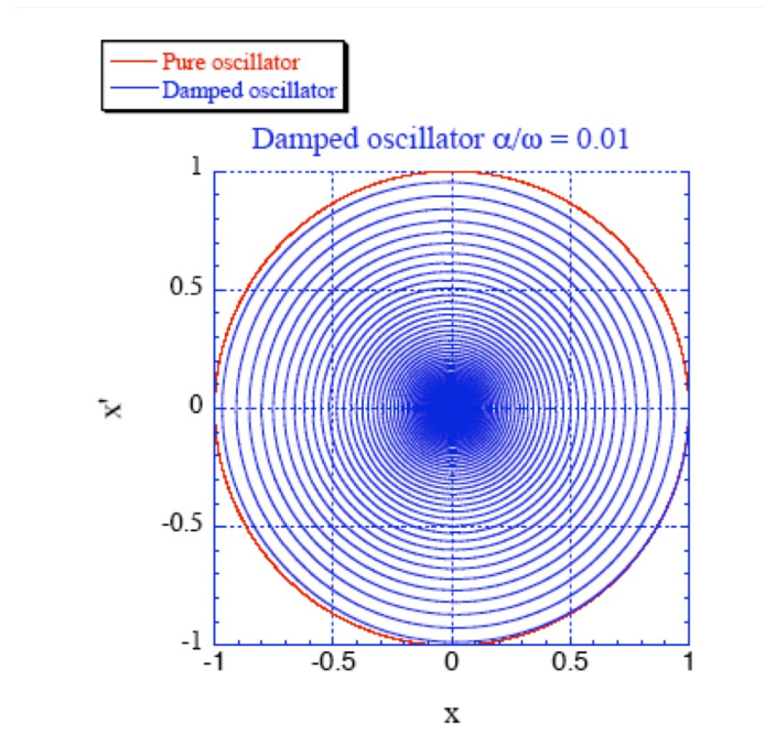
Fig. 1 Poincaré plot of trajectories of normal and damped oscillator in dimensionless coordinates x/a ; x'/\omega a .
